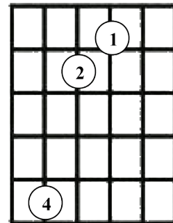
6 th Chord
