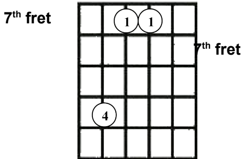
4 th Chord
