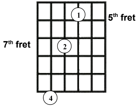
2 nd Chord
