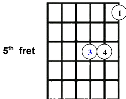
Major
