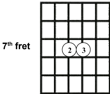
1 st Chord
