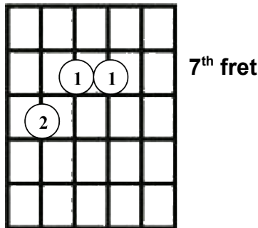
5 th Chord
