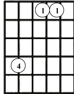
3 rd Chord
