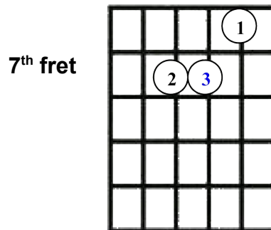
Minor
